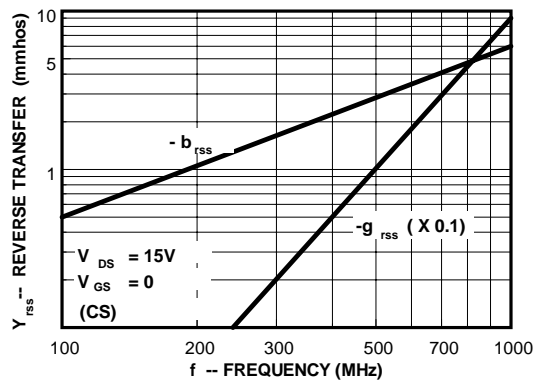
Reverse Transadmittance
